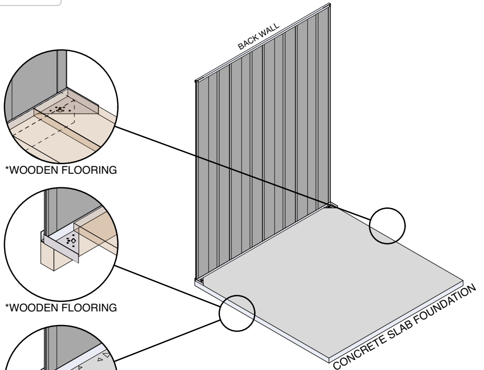
Corner Anchor x 4
